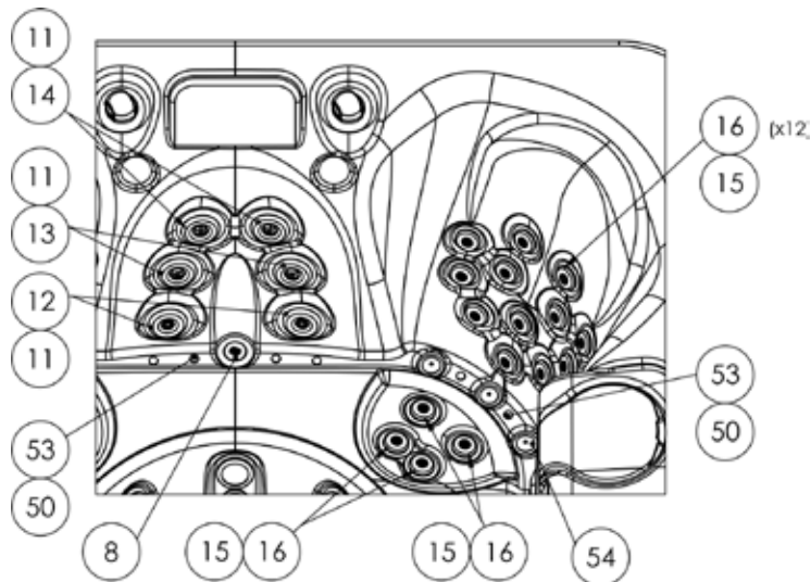
DETAIL D
